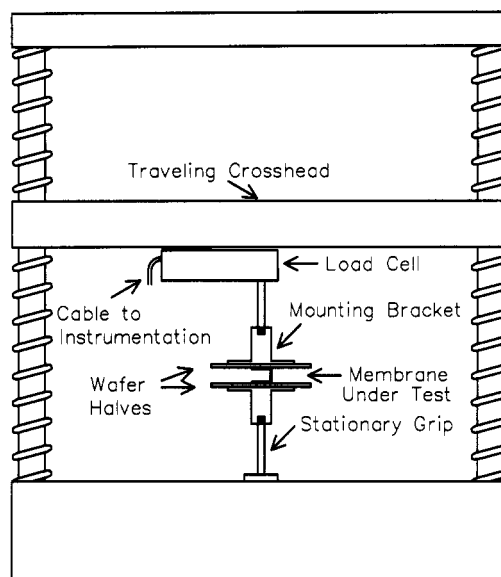
Figure 2. Schematic drawing of adhesion tester.
